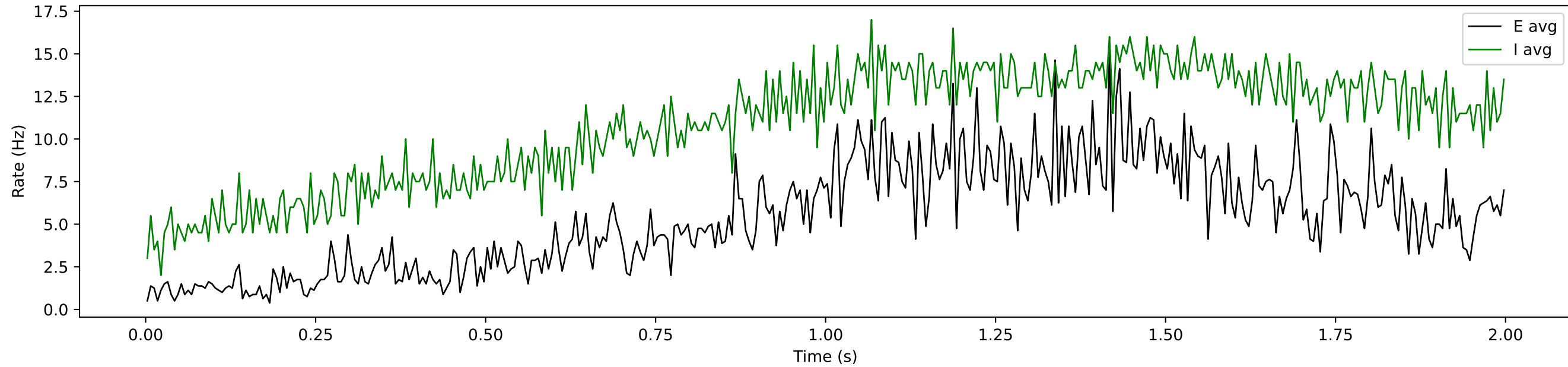
Population-Averaged Rates
